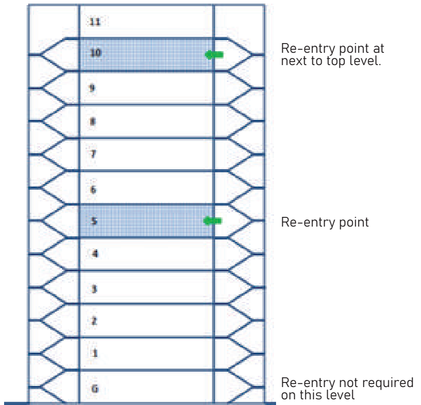
Figure 6.8.3.1 (b). Required re-entry floors when starting at the next to top level.
